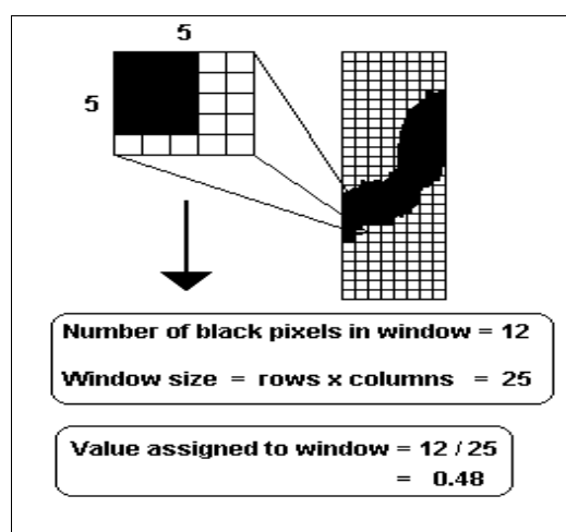
Figure 3. A window of 5x5 in dimension is extracted from a segmentation point matrix
