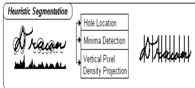
Figure 2. Heuristic Segmentation Algorithm
